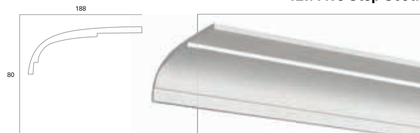
127. Five Step Scotia
