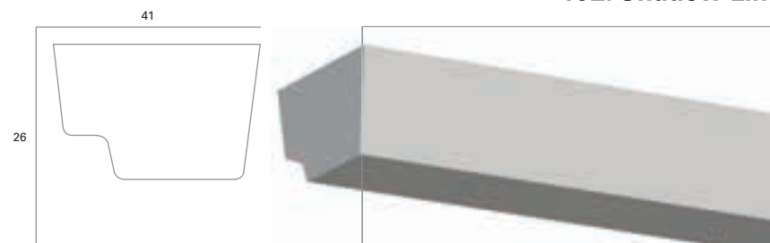
16E. Shadow Line
