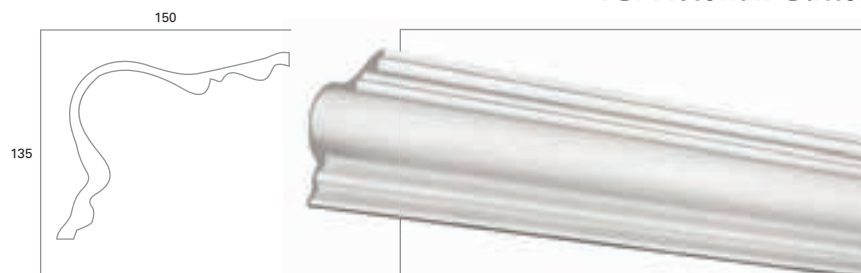
1G. Victorian Gutter
