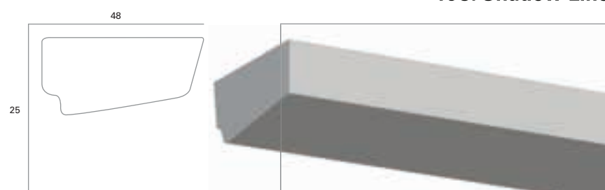
16C. Shadow Line
