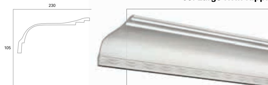
65. Large Twin Ripple
