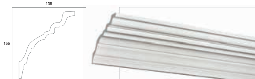
37C. Federation Glenlee
