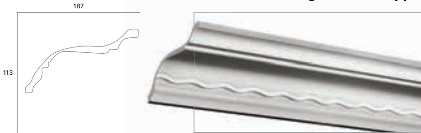
69. Large Double Ripple
